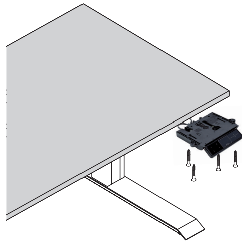
Abb. 31: Handschalter LegaData Drive Touch Comfort anbringen
