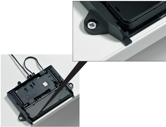
Abb. 29: Montageposition des Handschalters LegaData Drive Touch Comfort
