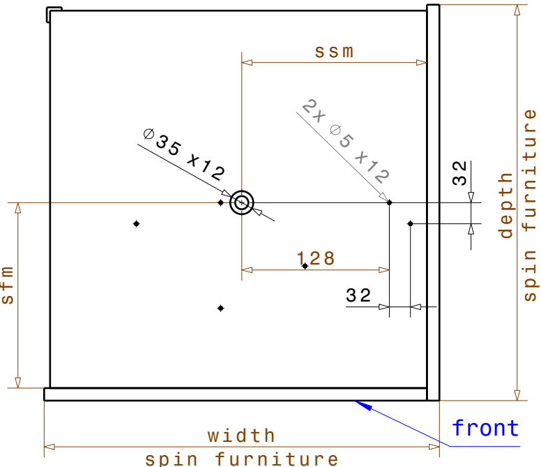
top panel/view 1:8
